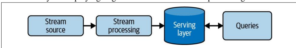
Figure 3-15. Kappa architecture
