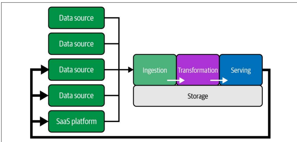
Figure 2-6. Reverse ETL
